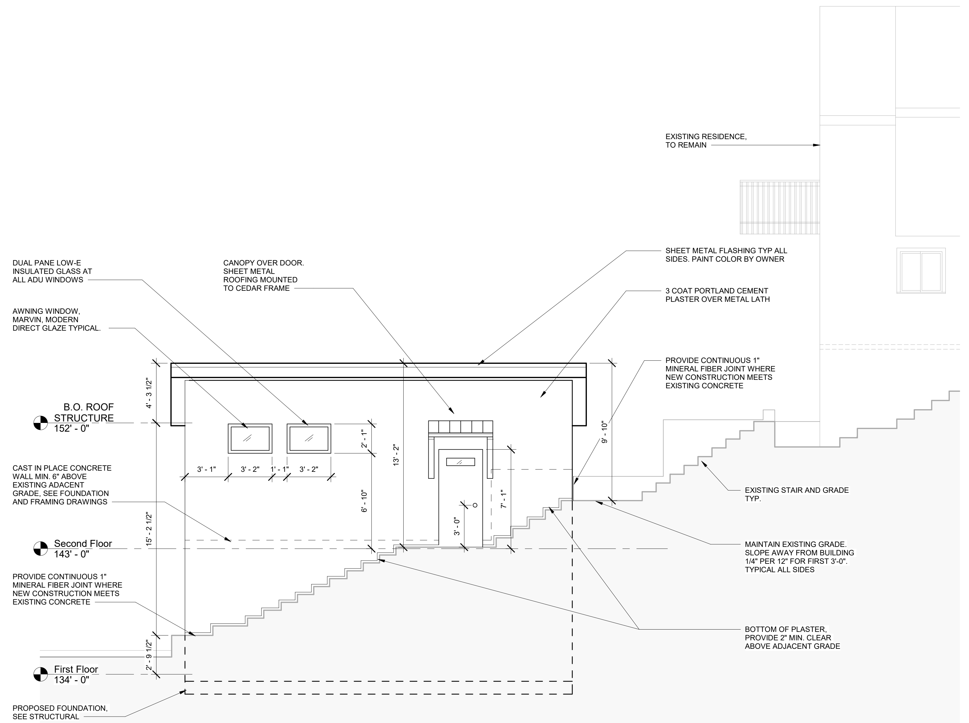
② West 1/4" = 1'-0"
