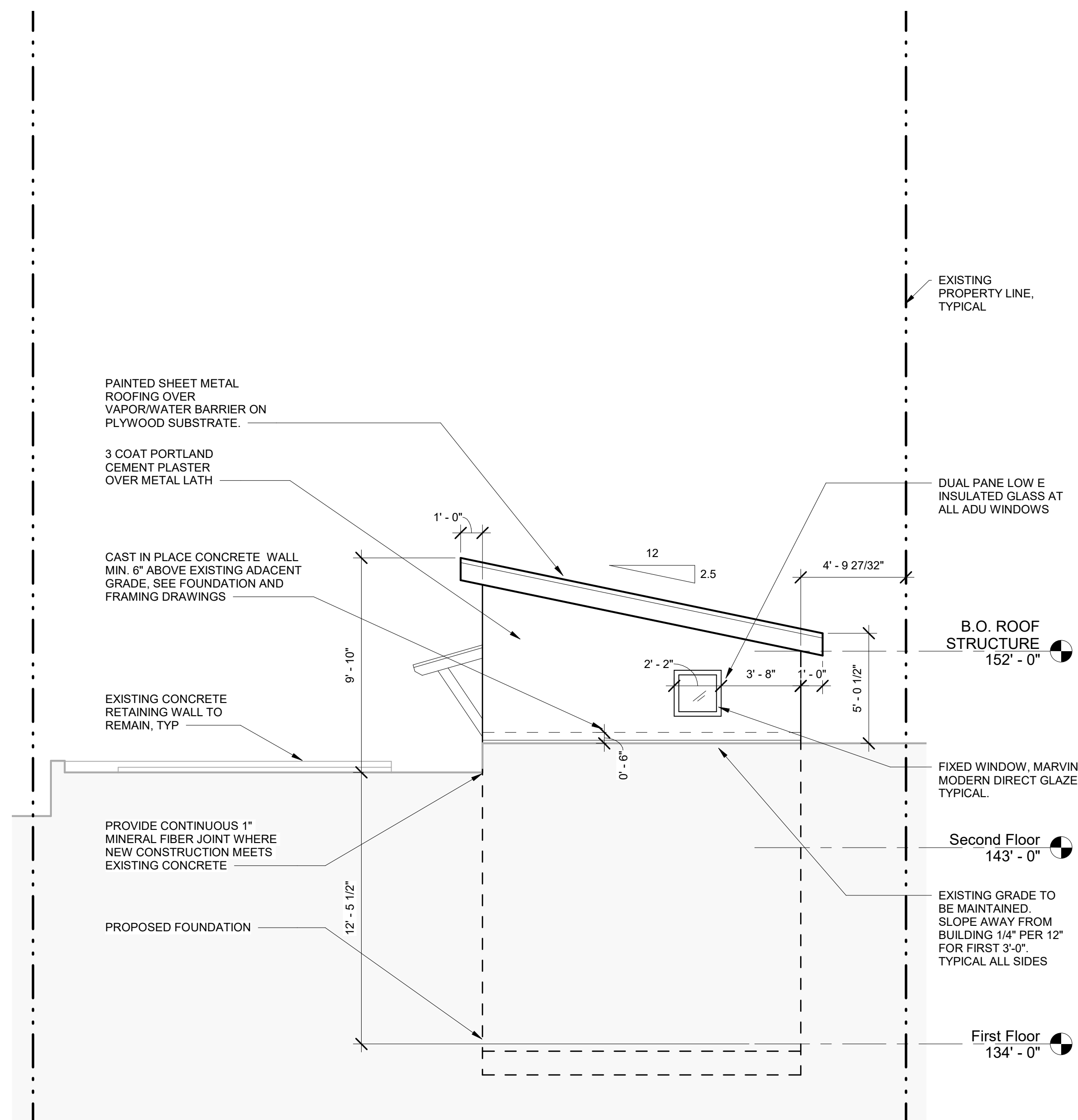
① South 1/4" = 1'-0"
